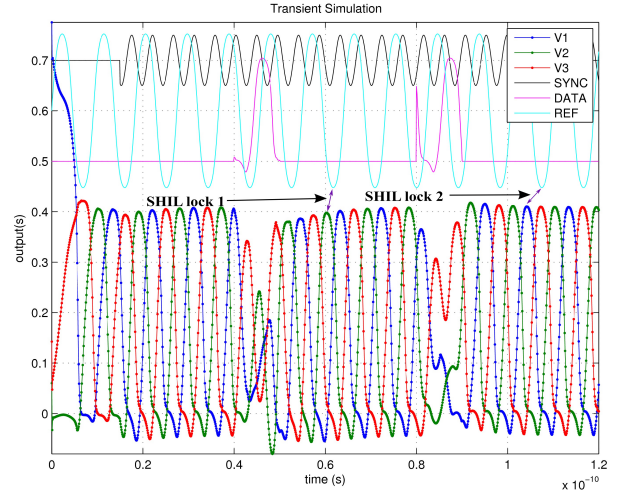
Fig. 3: Asymmetrized ring osc. transient simulation, showing two distinct SHIL lock states.
