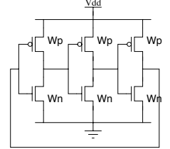
Fig. 1: 3-stage ring oscillator.
