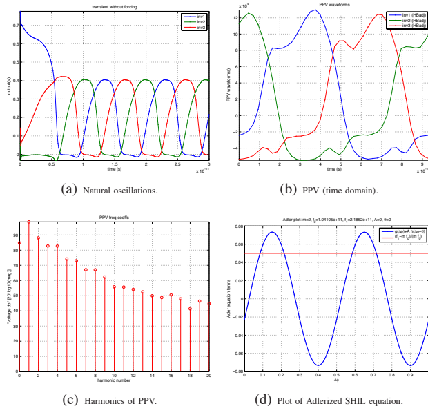
Fig. 2: Asymmetrized ring oscillator: natural oscillations, PPV waveforms and Adlerized SHIL plot.
