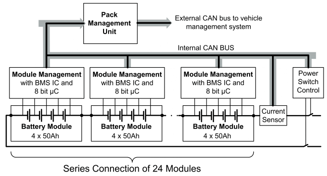
Figure 3. Battery system overview
