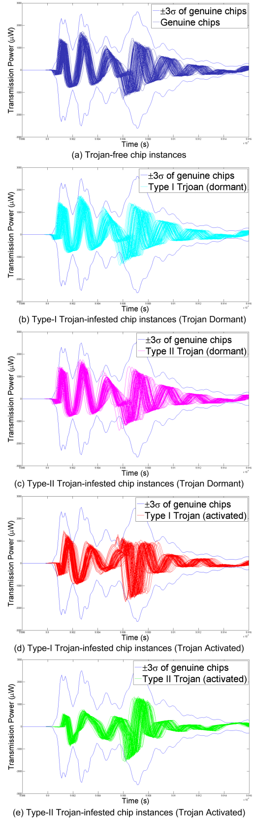
Fig. 6. \pm 3\sigma transmission power envelope of Trojan-free chip instances enclosing the various chip populations in our dataset
