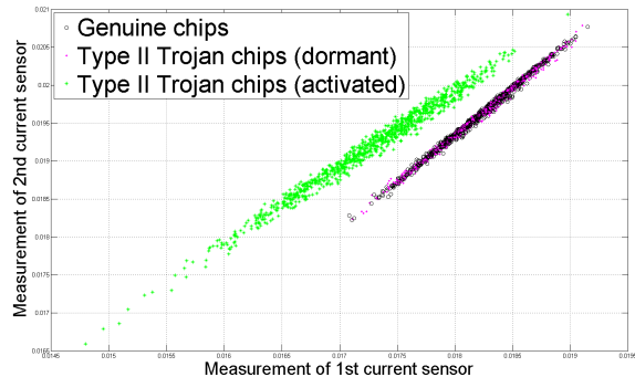
Fig. 9. Current sensor measurements for Type-II Trojan-infested chips
