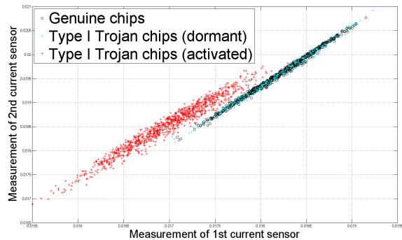
Fig. 8. Current sensor measurements for Type-I Trojan-infested chips
