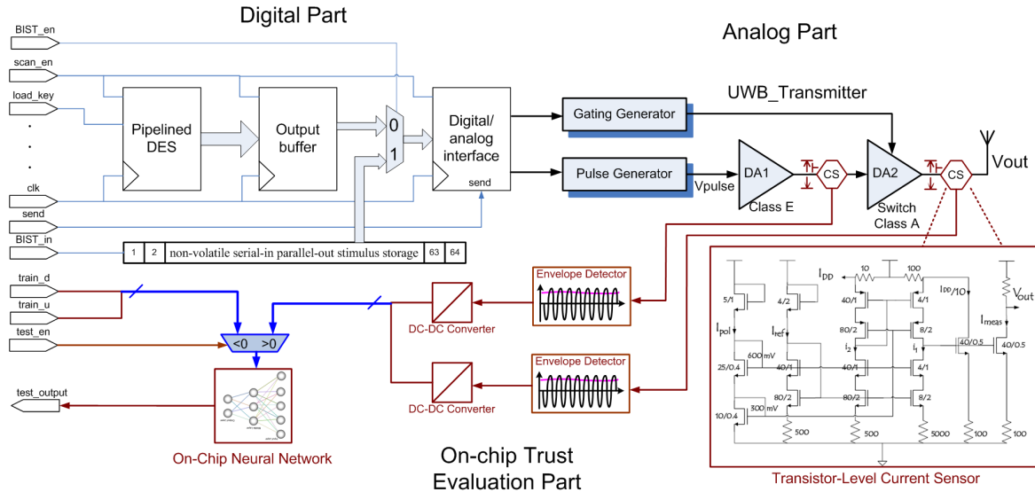
Fig. 2. Architecture of wireless cryptographic IC experimental platform
