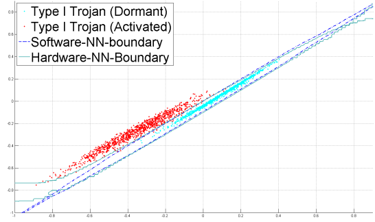
Fig. 11. Ability of boundary learned through software and hardware NN to correctly classify dormant and activated Type-I Trojan-infested chips
