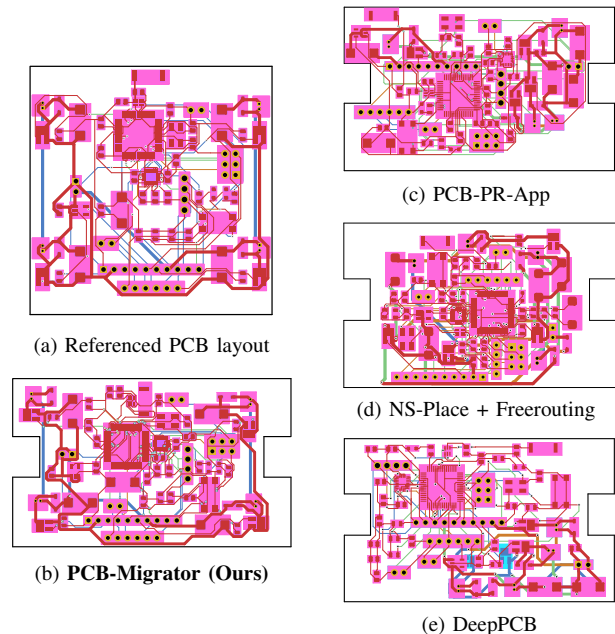
Fig. 9 Comparison between the referenced P5 layout and migrated layouts from our PCB-Migrator and other baselines. PCB-Migrator’s layout is highly similar to the reference and more reasonable, resulting in improved EM performance.
