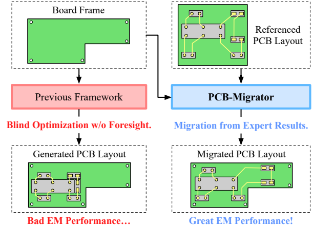
Fig. 1 Our PCB-Migrator compared with previous automated frameworks that design PCBs from scratch. Migration from expert results enables PCB-Migrator to have foresight in the early stage, thus enhancing its practical performance.
