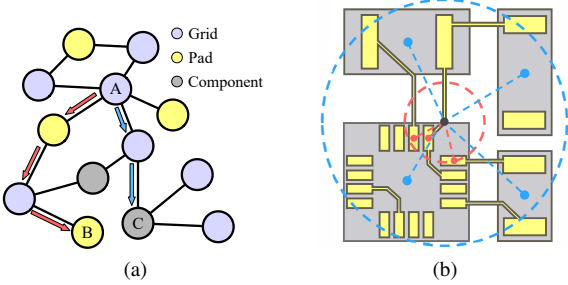
Fig. 6 (a) Example of neighborhood connection calculation. To the grid node A , 3 steps are required to reach pad node B (the red path), so the corresponding value is (t_p)^3 . Similarly, 2 steps are required to reach component node C (the blue path), so the corresponding value is (t_c)^2 . (b) Pad-dense area with fine-grained routing characteristics (shown in red). Regular routing area between components, with coarse-grained routing characteristics (shown in blue).
