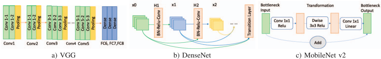
Fig. 1: Architectures of VGG, DenseNet, and MobileNet v2
