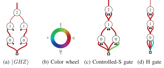
Fig. 2. Decision diagrams for 3-qubit states and gates
