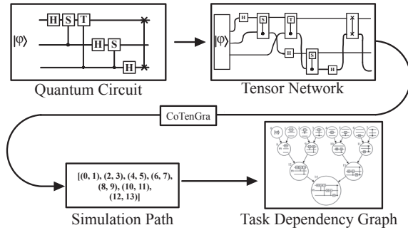
Fig. 4. Automated flow for determining simulation paths
