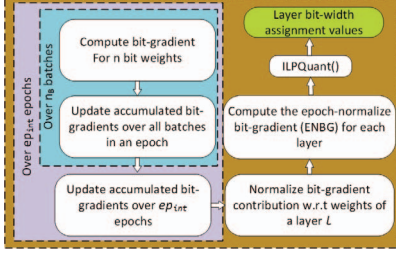
Fig. 1. Step-wise description of layer bit-width evaluation.
