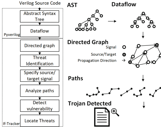
Fig. 1: Workflow of the proposed If-Tracker framework.
