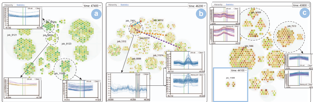
Fig. 3. The main view and corresponding detailed views of the visual analytics system. Detailed views of multiple line charts show the metric utilization trends of compute nodes under a selected batch job over time. The green annotation lines in each line chart depict the start timestamps of the selected job across each compute node executing it, while other annotation lines denote the job end timestamps using the same color as the corresponding lines of nodes.
