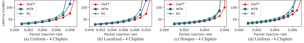
Figure 4. Average latency comparison among DeFT , MTR, and RC routing algorithms when applied to the network shown in Fig. 1 and under (a) Uniform, (b) Localized, and (c) Hotspot synthetic traffic patterns. (d) shows the same but for 6 chiplets and Uniform traffic.
