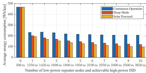
Fig. 2. Average energy consumption normalized to 1 km for the conventional cellular corridor and 1 to 10 low-power repeater nodes in between high-power masts to extend their ISD while maintaining the peak throughput for users.
