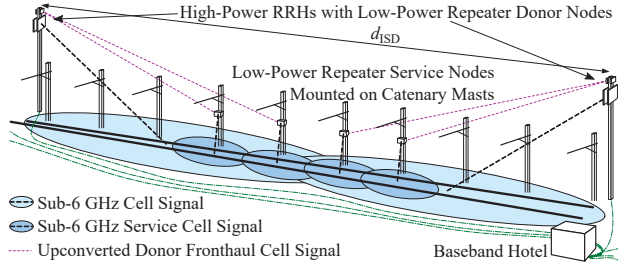
Fig. 1. Railway corridor with macro sites providing the linear cell enhanced by out-of-band amplify-and-forward repeater nodes in between.
