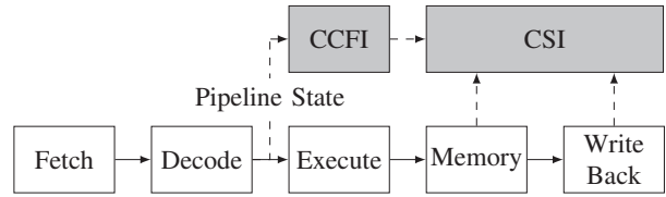
Fig. 1. Illustration of a 5-stage processor extended with SCI-FI (grey modules)
