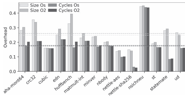
Fig. 2. Execution time and code size overheads for the Embench-IoT benchmarks, with the -Os and -O2 compiler optimization levels.
