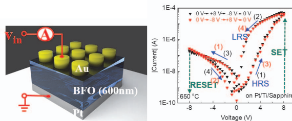
Fig. 4: BFO memristive device and its electrical behavior
