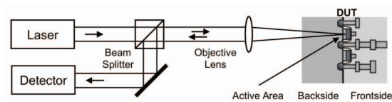
Fig. 5: Optical probing signal acquisition (simplified)
