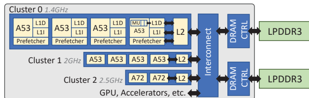
Fig. 1. Memory system organization of the MediaTek Helio X20 SoC.
