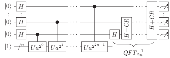
Fig. 2. Circuit blocks of Shor’s algorithm
