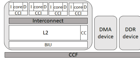
Fig. 1: Simplified block diagram of the T2080
