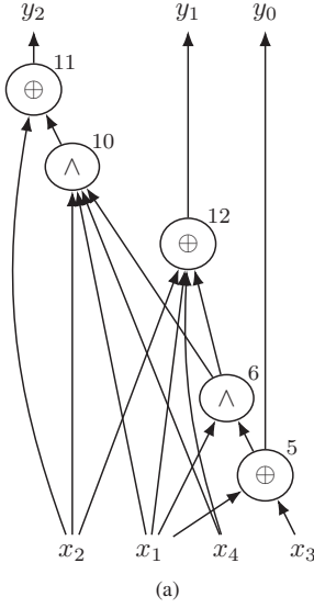
Fig. 1. Starting from the XAG, we first create a high-level XAG (a). We synthesize a quantum circuit with parity gates and Toffoli gates (b); Then we lower it to a circuit consisting of CNOT and Toffoli gates (c), which, in turn, is lowered to a circuit over the Clifford+ T gate set.
