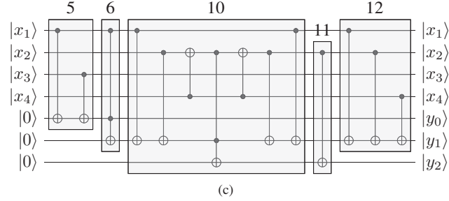
Fig. 1. Starting from the XAG, we first create a high-level XAG (a). We synthesize a quantum circuit with parity gates and Toffoli gates (b); Then we lower it to a circuit consisting of CNOT and Toffoli gates (c), which, in turn, is lowered to a circuit over the Clifford+ T gate set.
