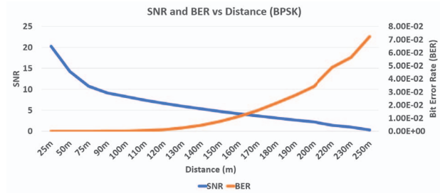
Fig. 3. SNR/BER vs distance for BPSK modulation with Friis prop. loss.
