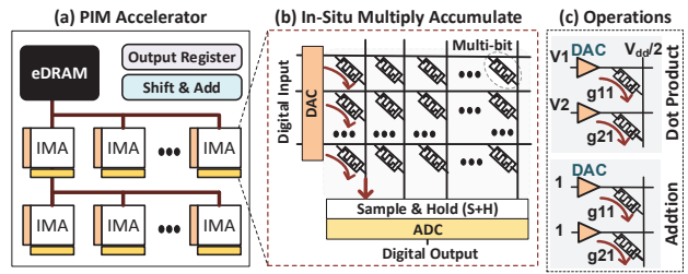
Fig. 1. Overview of the PIM architecture used by HyDREA
