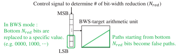
Fig. 2. Assumed BWS. In BWS operation, bottom bits will be replaced to the user-defined value. Paths starting from replaced bits become false paths and will not toggle in the arithmetic unit.
