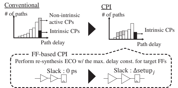
Fig. 3. Assumed FF-based CPI with re-synthesis.
