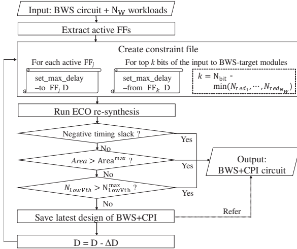
Fig. 4. Overview of the CPI flow.
