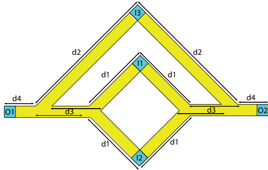
Fig. 3. Fan-out of 2 MAJ3 Gate.
