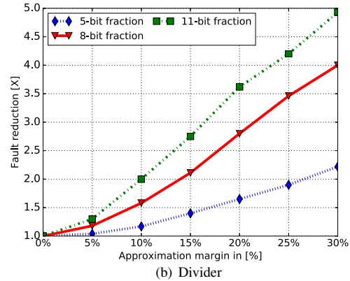
Fig. 4. Fault reduction of approximate fixed-point circuits for different levels of approximation margin and varying fractional bit widths
