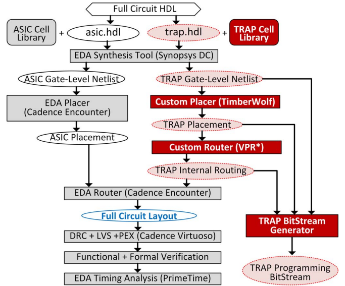
Fig. 4: CAD Tool-flow for TRAP-based Design Obfuscation.
