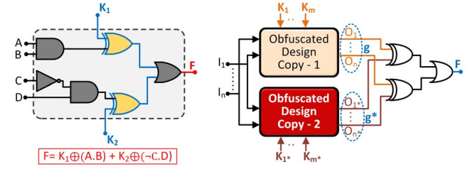
(a) Logic obfuscation example.
