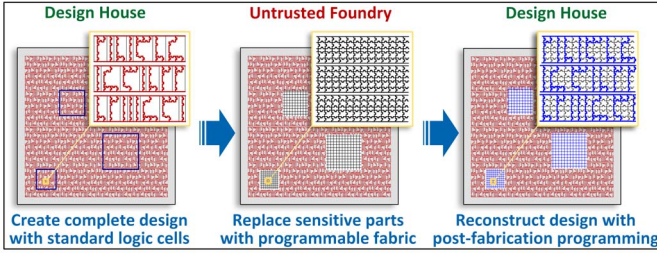
Fig. 1: TRAP-based design obfuscation.
