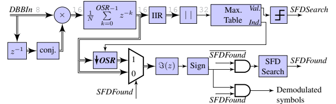
Fig. 3. Simplified view of FSK demodulation algorithm. Double arrows indicate complex signals. The signal dynamic range is shown in lighter type.
