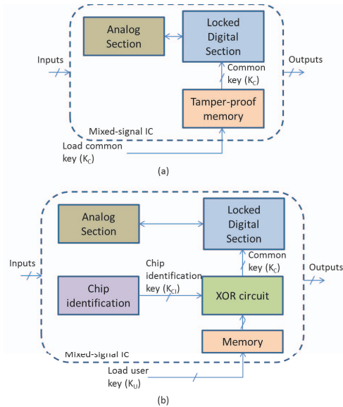
Fig. 1. Mixed-signal IC locked with MixLock .
