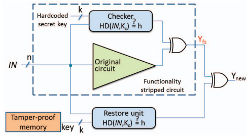
Fig. 2. SFL architecture.
