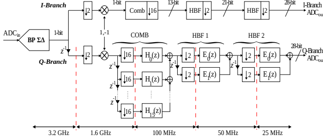
Fig. 5. The digital DDC mixer and decimation filter.
