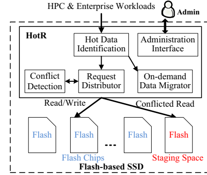
Fig. 2. System overview of HotR.
