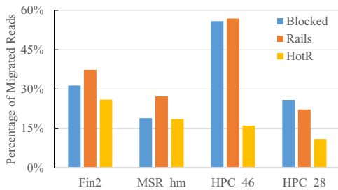
Fig. 6. The percentages of redirected read requests by the Rails and HotR schemes. The Blocked indicates the percentage of read requests that are blocked in the baseline system with no optimizations.
