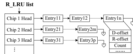
Fig. 3. The R-LRU data structure.
