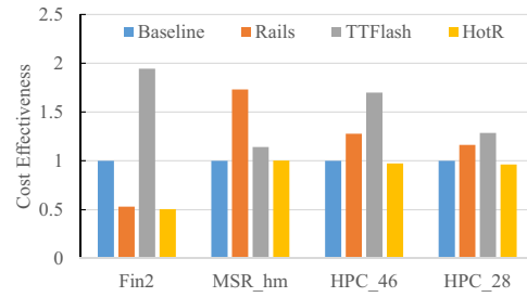
Fig. 7. The cost-effectiveness results of the difference schemes under the four workloads, normalized to the baseline system with no optimizations and space redundancy. Note that the lower the value, the better for the cost effectiveness.
