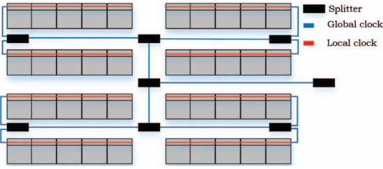
Fig. 1. A sample HL-tree clock network. Black boxes indicate clock splitters. Blue and red lines denote the global and local clock signals.
