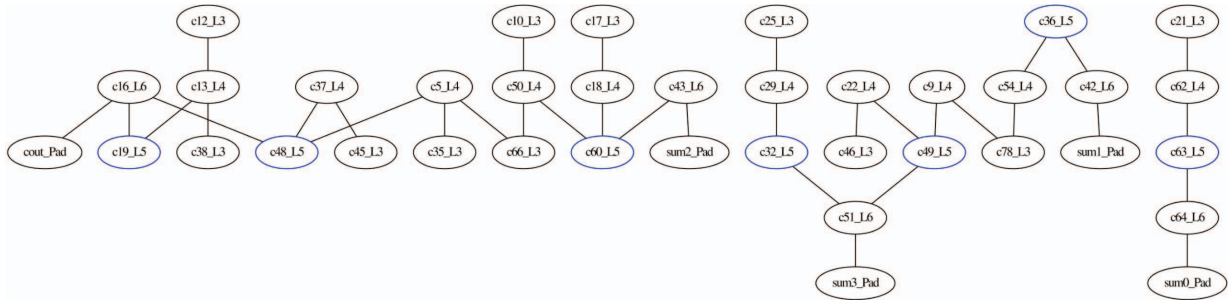
Fig. 3. Graph of nodes of level 3-6 for a 4-bit Kogge-Stone adder. Nodes of level 5 are shown in blue. Logic level of each node is added to its name.
