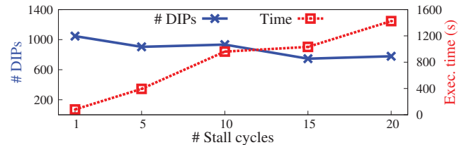
Fig. 7. Effect of stall cycles on security for a fixed key size of 14 bits. which acts as a threshold. Since for performance locking the error rate is \frac{1}{2^k} , the attack terminates within a few seconds. Yet, it fails to extract the correct key.
