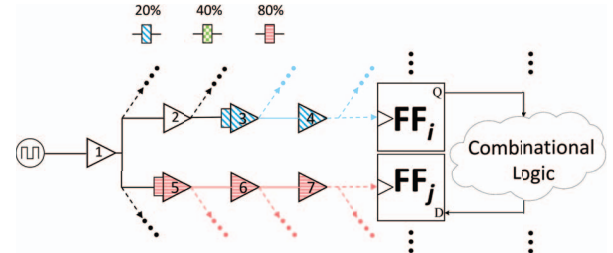
(b) Case 2-2: one DCC on one of the divergent clock paths, or class 3: two DCCs, one on each of the divergent clock paths
