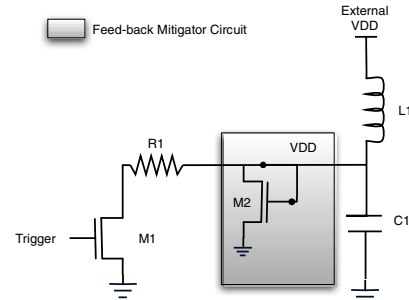
Fig.2: Feedback based droop mitigation
