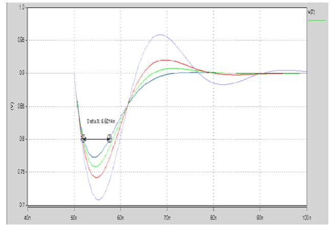
Fig. 4: comparison of droop mitigation at different W
