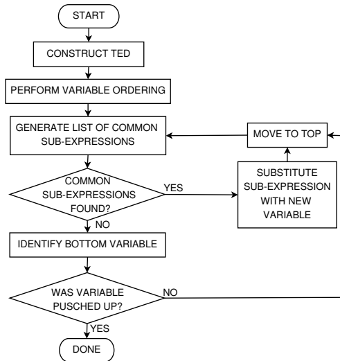
Figure 2. Flow chart of the CSE algorithm
