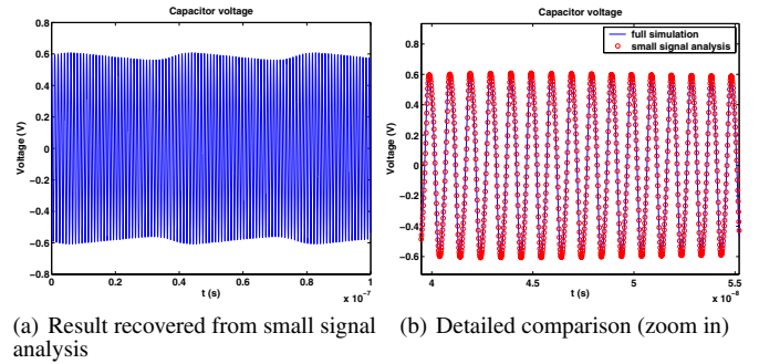
Fig. 10. Comparison of results from small signal analysis and full transient simulation.
