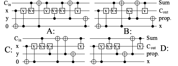
Figure 2. Simplification of a 10-gate quantum network for the 3-bit full adder.
