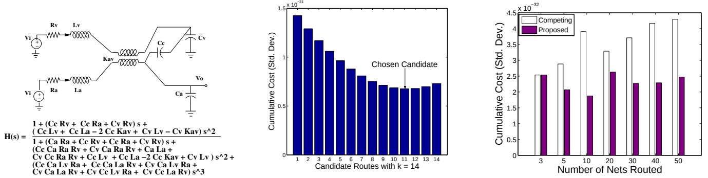
Figure 1. (A) Transfer function of 2 coupled wires (B) Possible Candidate Routes (C) Cumulative Cost comparison
