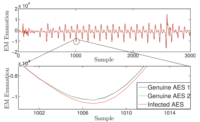
Figure 5. Hardware trojan detection using averaged EM traces
