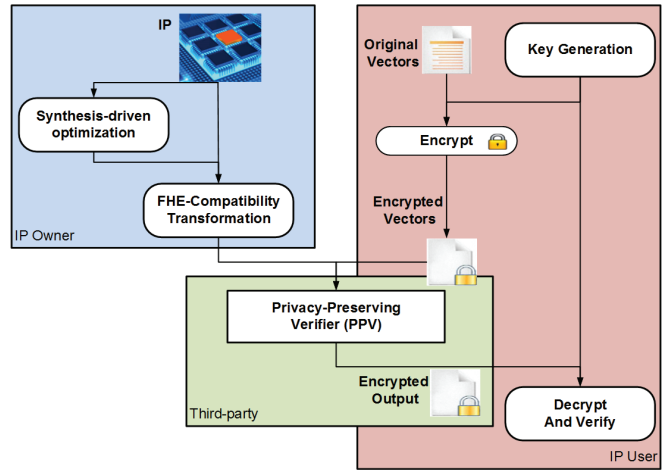
Fig. 1. Flowchart of the privacy-preserving verification protocol
