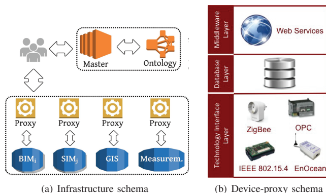
Fig. 1. Depiction of the whole infrastructure (a) and the Device-proxy (b)
