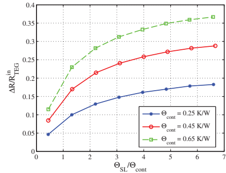
Fig. 5. Sensitivity analysis of resistance mismatch ratio on the TEG contact and super-lattice thermal resistivity
