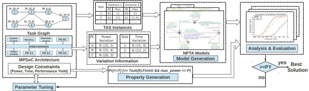
Fig. 3. Our TAS strategy evaluation framework
