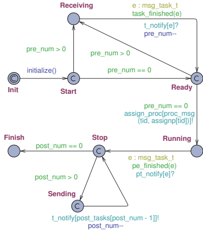
Fig. 4. Front-end model of a task
