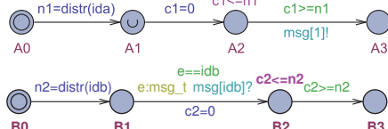
Fig. 1. An NPTA, ( A \mid B )
