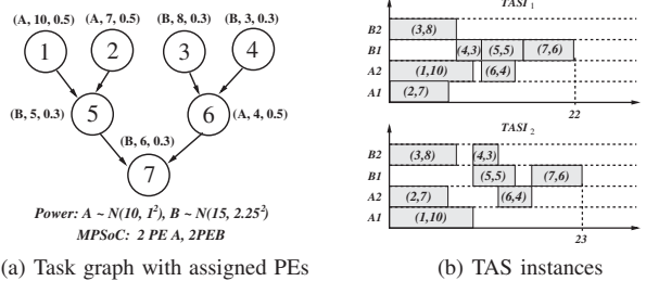
Fig. 2. A TAS problem and its two TAS instances
