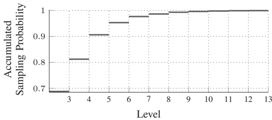
Fig. 2. The probability that the Knuth-Yao sampling algorithm finds a terminal node within x levels for a Gaussian distribution with \sigma = 11.31/\sqrt{2\pi} .
