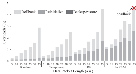
Fig. 9. I/O overheads vs. data packet length.
