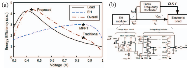
Fig. 10. Maximum energy efficiency tracking for converter-less systems [58].
