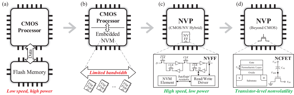
Fig. 2. Evolution of NVP.
