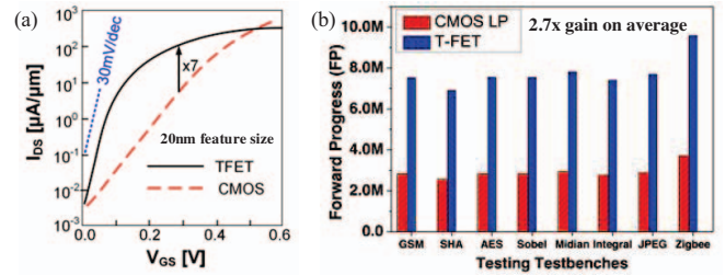
Fig. 3. (a) TFET I_{DS} - V_{GS} in comparison with CMOS [28]–[30]. (b) Forward progress improvement with TFET logic of MiBench testbenches powered with ambient RF energy [31].
