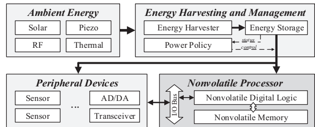
Fig. 1. NVP: the heart of energy harvesting IoT platform [14]–[16].
