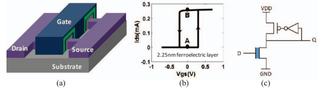
Fig. 4. Nonvolatile computing with NCFET. (a) NCFET in a fin structure [35]. (b) NCFET device drain current versus gate driving voltage [33]. (c) NCFET logic with logic-memory synergy.
