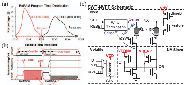
Fig. 7. Self-write-termination NVFF [27].
