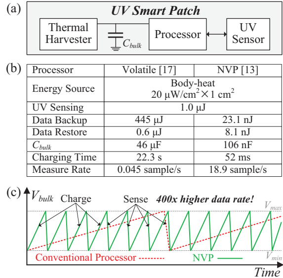
Fig. 5. Case study: a body-heat powered UV smart patch.
