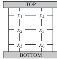
Fig. 4. Four-terminal switch based array/lattice implementing the Boolean function x_1x_2x_3 + x_1x_2x_5x_6 + x_2x_3x_4x_5 + x_4x_5x_6 .
