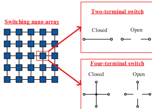
Fig. 1. A switching crossbar nanoarray modeled with two-terminal and four-terminal switches.
