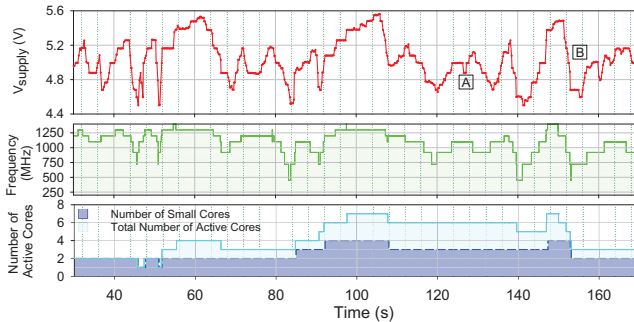
Fig. 11. System performance using a controlled variable voltage supply. Parameters V_{width}=335mV ; V_q=190mV ; \alpha=0.238Vs^{-1} ; \beta=0.633Vs^{-1} .
