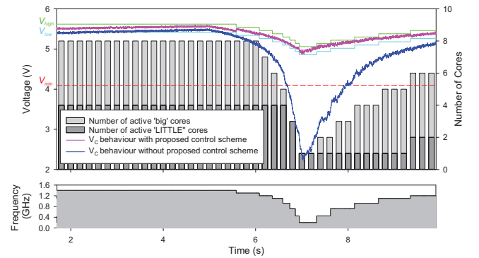
Fig. 6. Simulation showing operation of the control algorithm. Parameters V_{width}=0.2V ; V_q=80mV ; \alpha=0.1Vs^{-1} ; and \beta=0.12Vs^{-1} .
