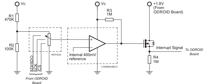
Fig. 9. Schematic of the voltage monitoring hardware.
