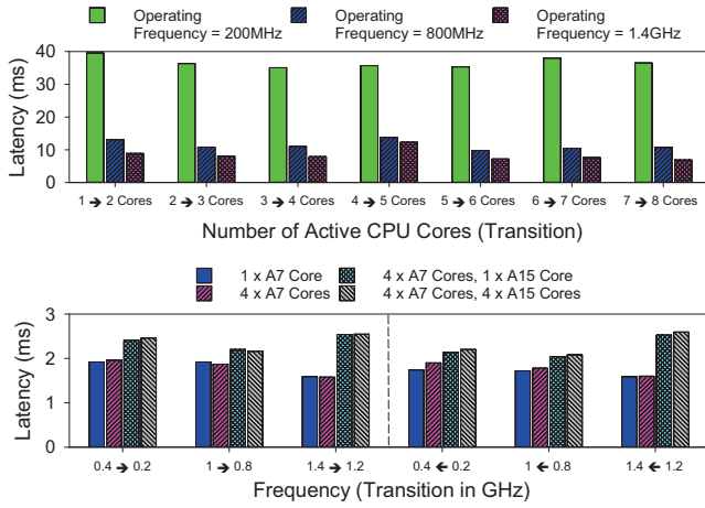
Fig. 10. Latency to switch number of active CPU cores using hot-plugging (top) and to change the operating frequency (bottom), obtained experimentally for the ODROID XU4 SoC platform.
