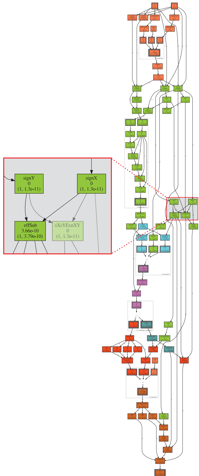
Fig. 5: S-Graph for a single-precision floating-point adder
