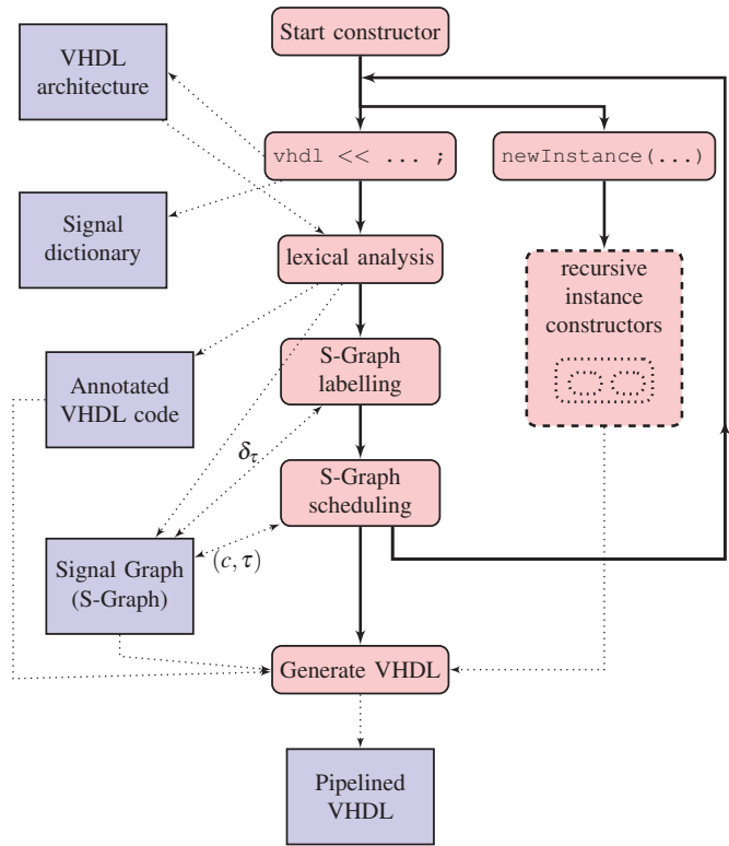
Fig. 2: Constructor flow overview
