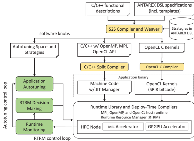
Fig. 1. The ANTAREX Tool Flow
