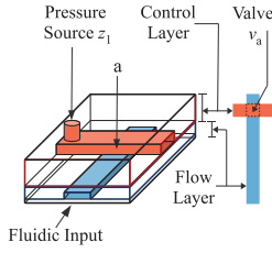
Figure 1. Structure of a valve fabricated using soft lithography
