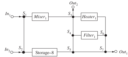
Figure 3. Biochip architecture example
