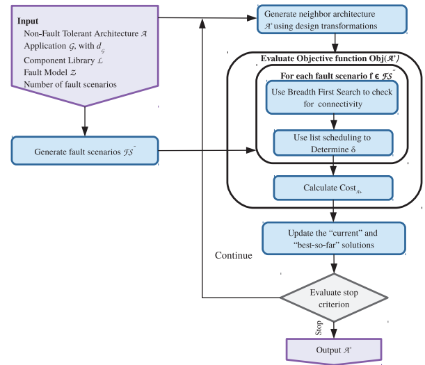
Figure 6. Fault Tolerant Architecture Synthesis (FTAS)
