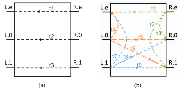
Fig. 5: Pre-inserted pipeline buffer: (a) Transparent mode (b) Opaque mode
