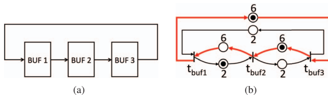
Fig. 1: (a) Three-stage pipeline. (b) FBCN model.
