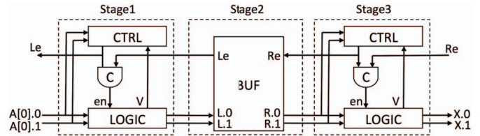
Fig. 4: A three-stage PCHB pipeline.
