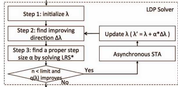
Fig. 7: Lagrangian dual problem solver.
