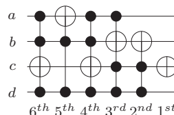
Fig. 1: Circuit obtained by transformation-based synthesis
