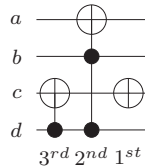
Fig. 2: Res. circuit
