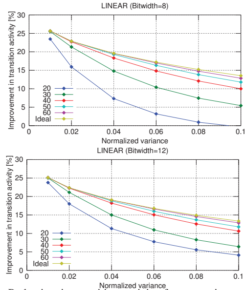
Fig. 5: Reduction in transition activity for approximate encoders using between 20% and 60% of the patterns. Reduction analysed versus the statistical characteristics of the input PDF
