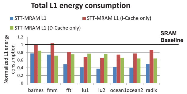
Fig. 6. MRAM-based L1 energy consumption
