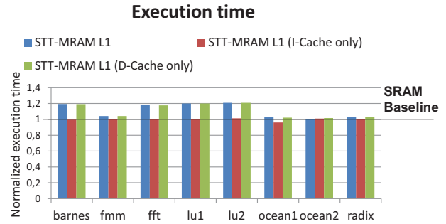
Fig. 5. Execution time of MRAM-based L1 cache
