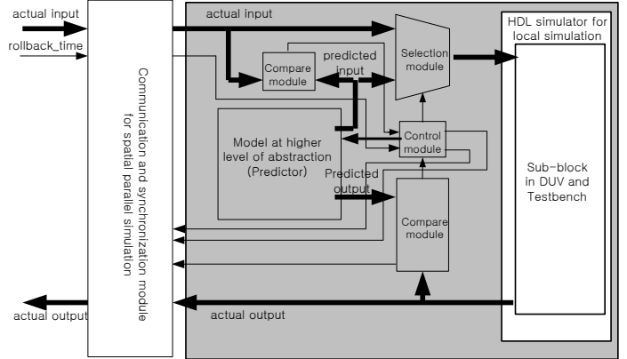
Figure 3. Detailed architecture for local simulation.
