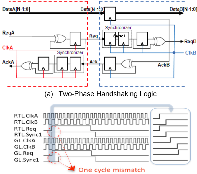
Figure 4. Two-Phase Handshaking Logic.
