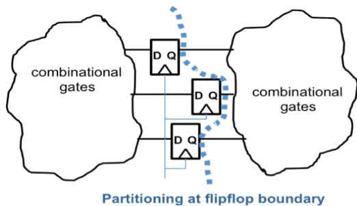
Figure 2. Partitioning scheme for accurate prediction.
