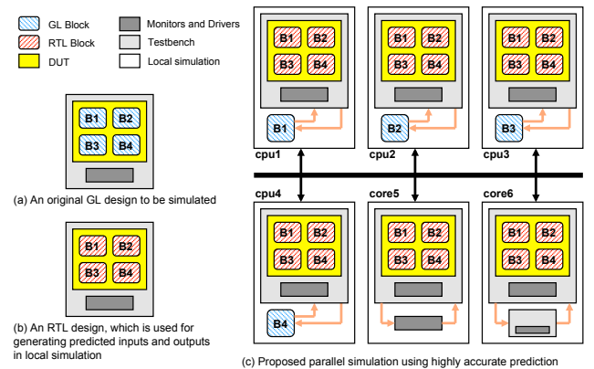
Figure 1. Basic concept of the proposed parallel event-driven HDL simulation using highly accurate prediction.
