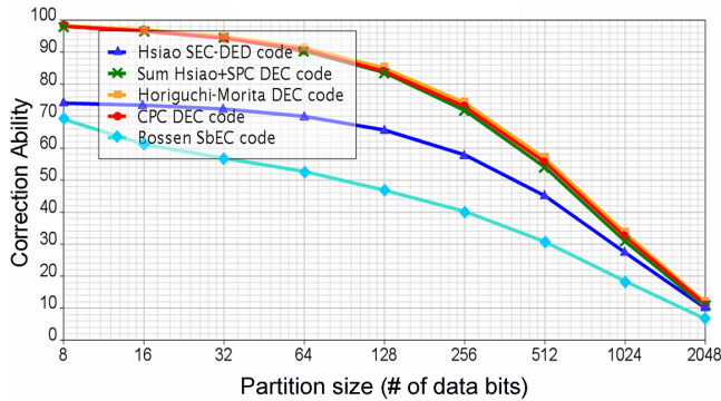
Fig. 3. Considered ECCs' correction ability comparison.
