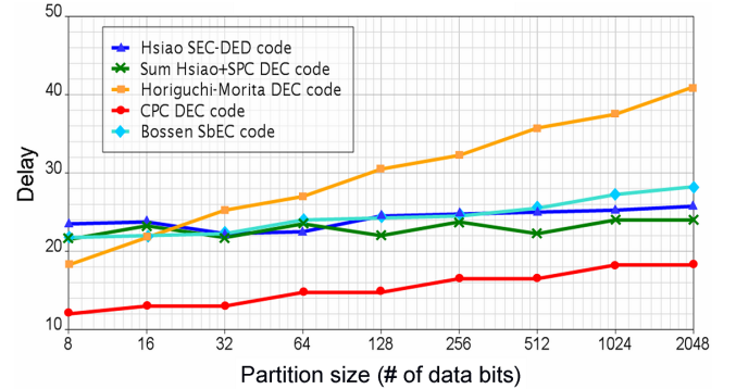
Fig. 1. Considered ECCs' delay comparison.
